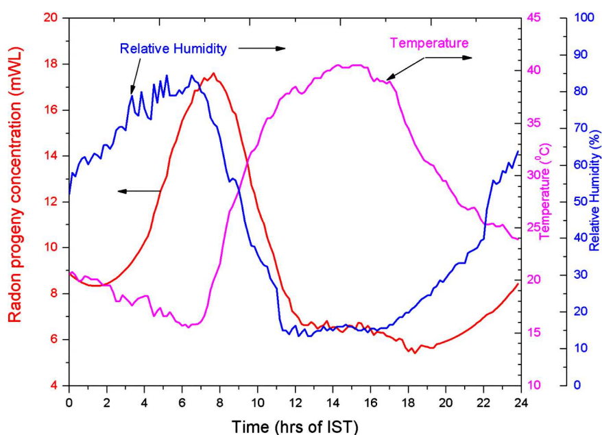
Figure 4. Variations of radon progeny concentration with ambient temperature and relative humidity.
