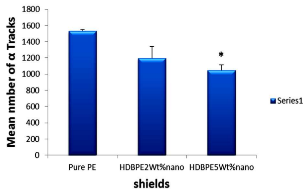
Figure 2. Mean number of \alpha tracks in different shields. Error bar shows the Standard Error. *Mean \pm SD of pure polyethylene and borated polyethylene nanocomposite there are significant differences.
