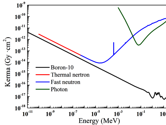
Figure 5. Energy-dependent kerma factors based on 1-ppm 10 B for neutron reactions with 10 B, thermal neutron, fast neutron, and photon (18) .
