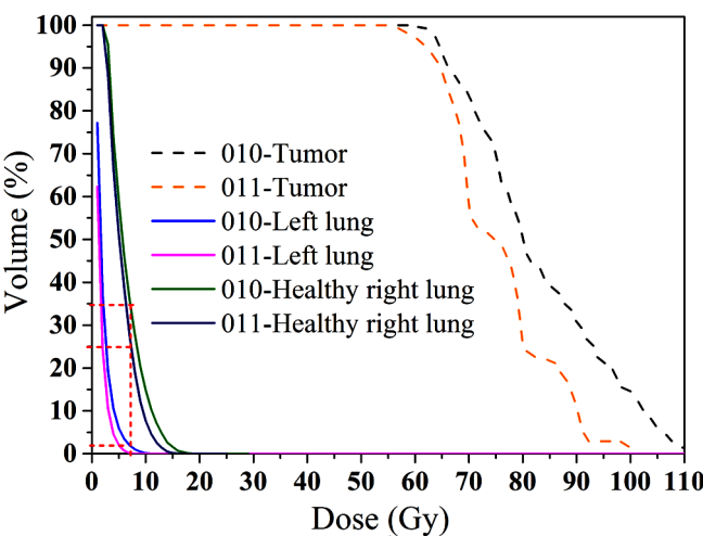
Figure 6. Considering 30/9 ppm of Boron-10 concentration in tumor/skin, dose in tumor, left lung and right healthy lung irradiated with plan (010) and plan (011).
