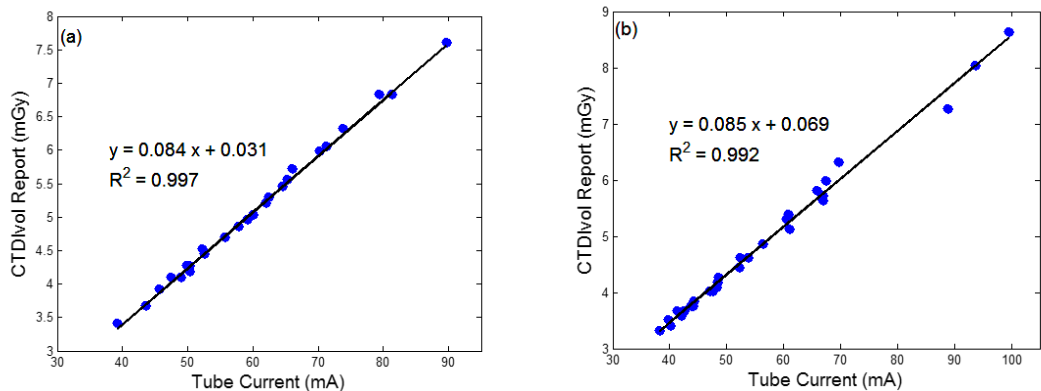
Figure 6. The relationships between average tube current and reported CTDI vol by scanner for (a) abdomen and (b) thorax.
