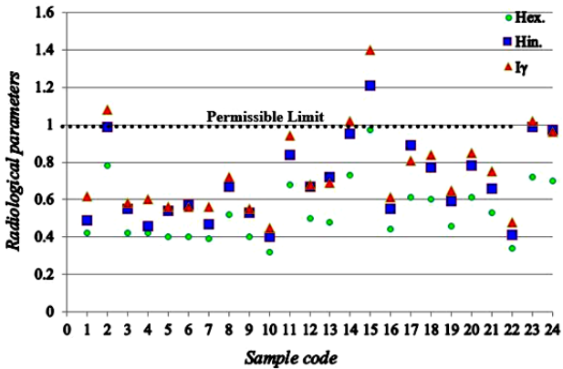
Figure 2. Relation between Radiological hazards with world limit.
