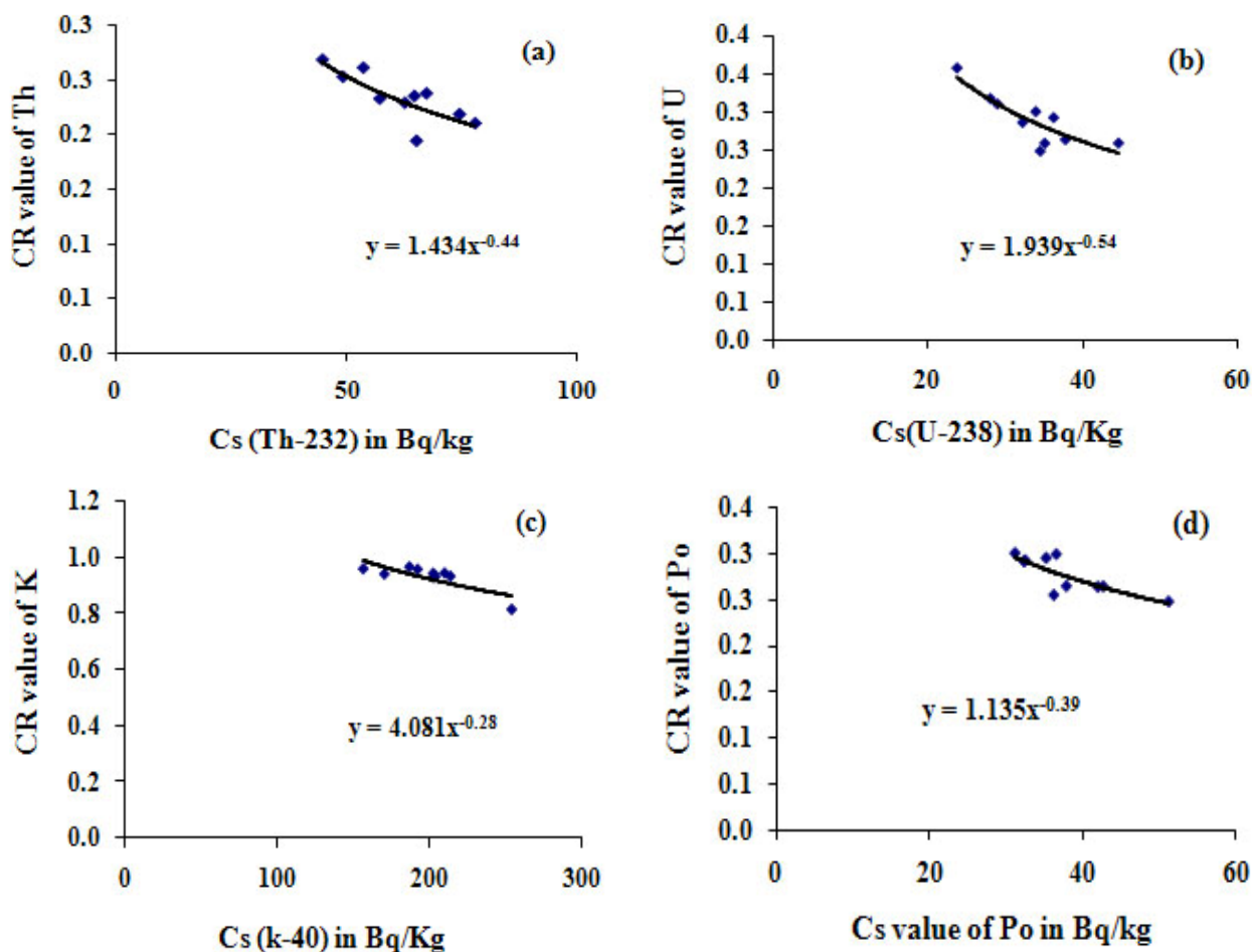
Figure 6. CR value vs. Cs of different radionuclides in soil for the plant of Evodia Roxburghiana .
