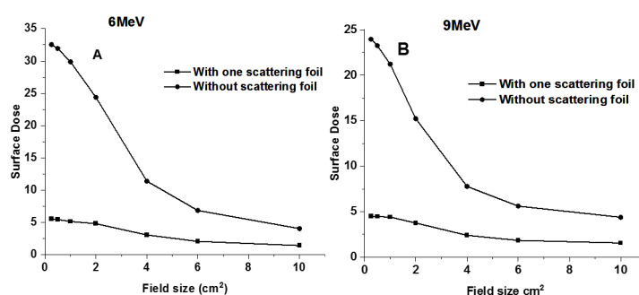
Figure 5. The increased surface dose for PSFF and SFF modes; (A) 6 MeV, (B) 9 MeV.
