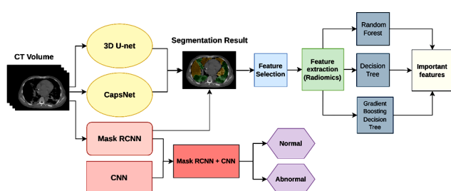
Figure 2. A detailed block diagram of the study in classification of COVID-19 lung disease and effective features extraction.
