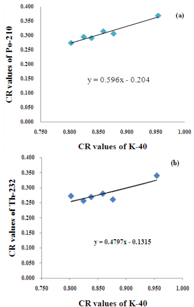
Figure 2. Correlation between CR values of different Radionuclides (a - ^{210}\text{Po} , b - ^{232}\text{Th} ) vs. ^{40}\text{K} .
