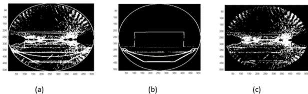
Figure 2. The scattering pattern caused by high-density structures (a). The pattern of high-density structures other than metal (b). The main pattern obtained by removing the other patterns from the scattering pattern (c). Lateral axis: x axis, vertical axis: z axis)
