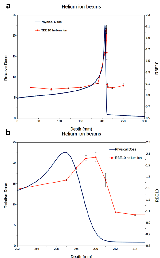
Figure 8. (a) RBE10 distribution of mono-energetic 176.4 MeV/ \mu m helium ion beams as a function of depth in a water phantom (b) zoom view.
