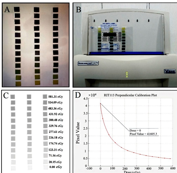
Figure 2. (A) The template of calibration films consists of 39 films of 1.5×1.5 cm 2 in 13 groups of 3 irradiated with specified prescribed doses in the dose range 0-570 cGy. (B) Scanning a template film with a Vidar scanner. (C) The scanned image of the calibration films labeled with the doses measured with the Exradin A1SL ionization chamber. (D) The Gafchromic EBT3 film calibration curve from the RIT software.
