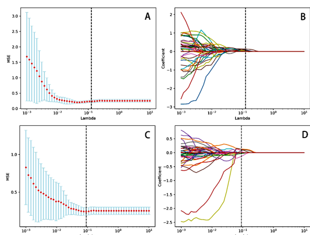
Figure 3. LASSO (least absolute shrinkage and selection operator) regression process. LASSO regression was used for radiomics feature selection, and the best lambda ( \lambda ) value was selected by tenfold cross-validation. In the figure, the ordinate "MSE" represents the mean square error, the ordinate "coefficient" refers to the radiomics feature coefficient, and the error bars is the standard deviation. (A) and (B) represent PET radiomics feature screening, and the best \lambda value is 0.125893, which is indicated by a dashed line. Similarly, (C) and (D) indicate CT radiomics feature extraction, and the best \lambda value is 0.091030.
