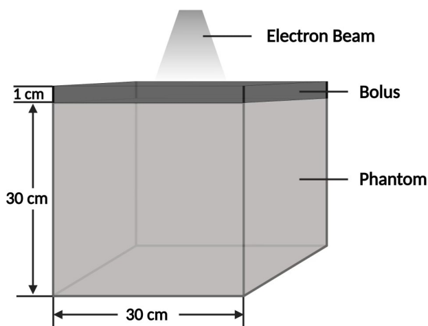
Figure 1. Model of electron beam irradiation.
