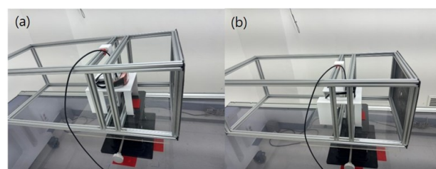
Figure 2. Measurements of radiation dose attenuation rates for lead glass of various thicknesses. All were conducted in accordance with the IEC 61331-1 standard. The experiment was designed to evaluate how different lead-equivalent thicknesses affect the shielding performance of goggles against scattered radiation. Distances, exposure conditions, and position measurements were performed as specified by the IEC guidelines: (a) the image represents the experimental setting, (b) the image represents actual settings according to the IEC guidelines and includes a 20 mm hole to narrow the beam width.
