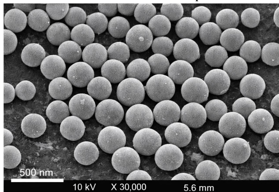
Figure 1. Scanning electron micrograph of hydroxyurea-loaded PLGA nanoparticles.
