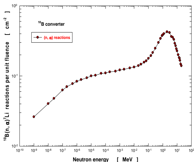
Figure 3. 10 B converter (n, α) response.
