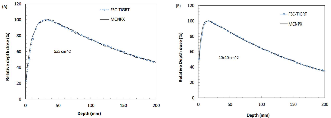
Figure 2. The comparison of relative depth doses from Monte Carlo Method and measurement in homogenous water phantom for two field sizes of (A) 5x5 and (B) 10x10 cm 2 for the 6 MV photon beam.
