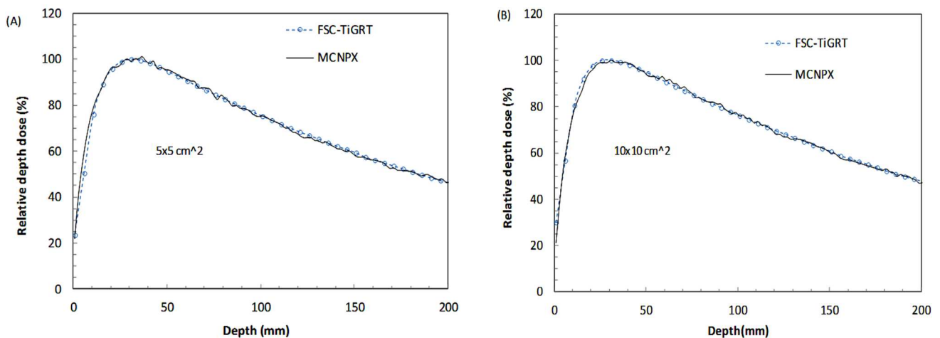
Figure 3. The comparison of relative depth doses from measurements and Monte Carlo Method in homogenous water phantom for two field sizes of (A) 5x5 and (B) 10x10 cm 2 for the 18 MV photon beam.
