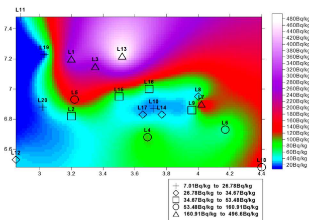
Figure 4. The image map of 40 K activity concentration for the study area.
