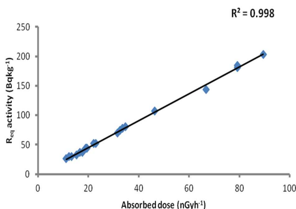
Figure 5. Variation of absorbed dose with Ra eq activity.
