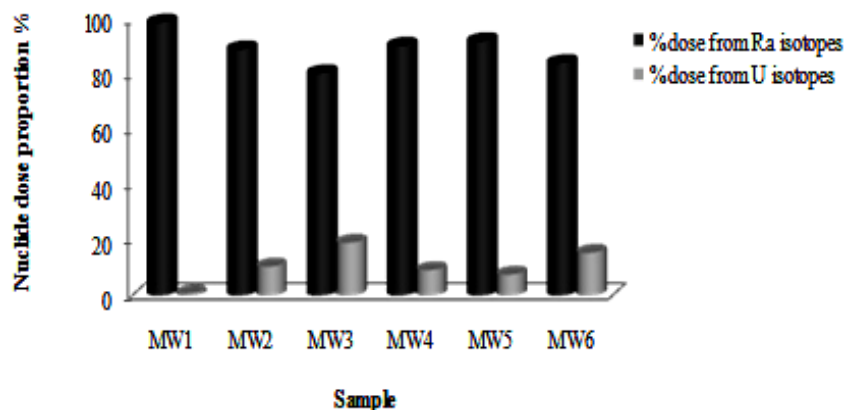
Figure 5. Percentage contribution of Ra and U isotopes to the total annual effective dose for adults (> 17 years) due to the intake of bottled mineral water.
