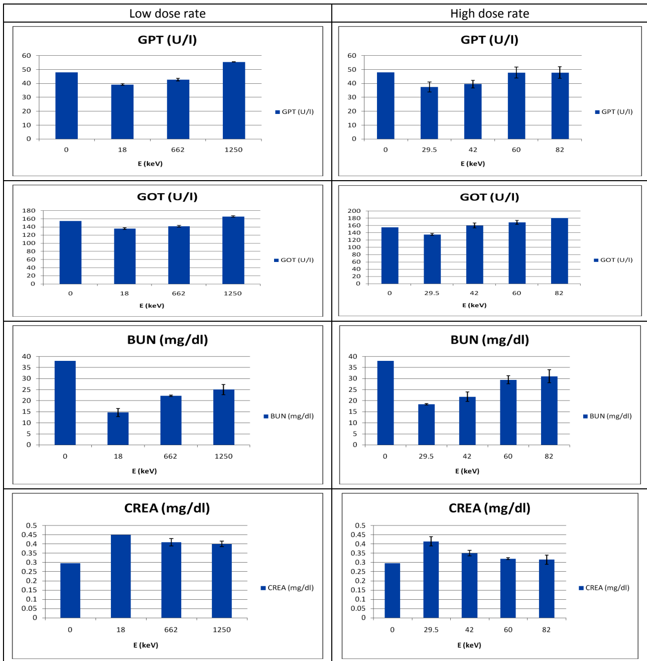
Figure 2. Representation for the SGPT, SGOT, BUN, CREA, Ca++ and CPK levels in blood for rats exposed to same dose with different energies.
