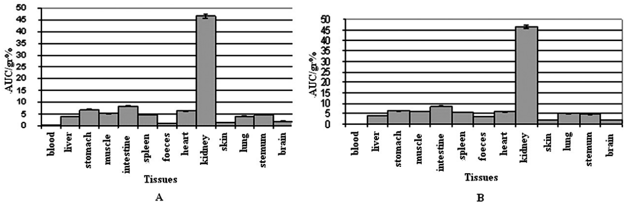
Figure 5. Bio-distribution of [ 201 Tl](III)-DTPA-HlgG in normal rats 20 (A) and 24 h (B) post-injection, (AUC: area under the curve of 167 keV peak) (n=5).
