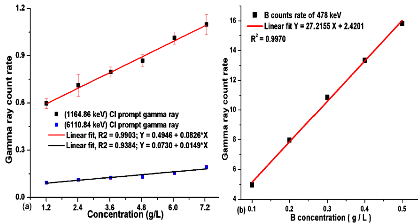
Figure 7. (a). Linear response for chlorine (calibration curve) (b) Boron with characteristic prompt gamma ray energies.
