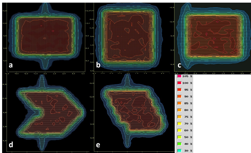
Figure 1. Beams of view of isodose curves measured for square field 5x5, Position of the contact of the closed leaves at (a) X=0. (b) X=-2.5. (c) X=-10. (d) and (e) irregular fields of 25 cm², Position of the contact of the closed leaves at X=0.
