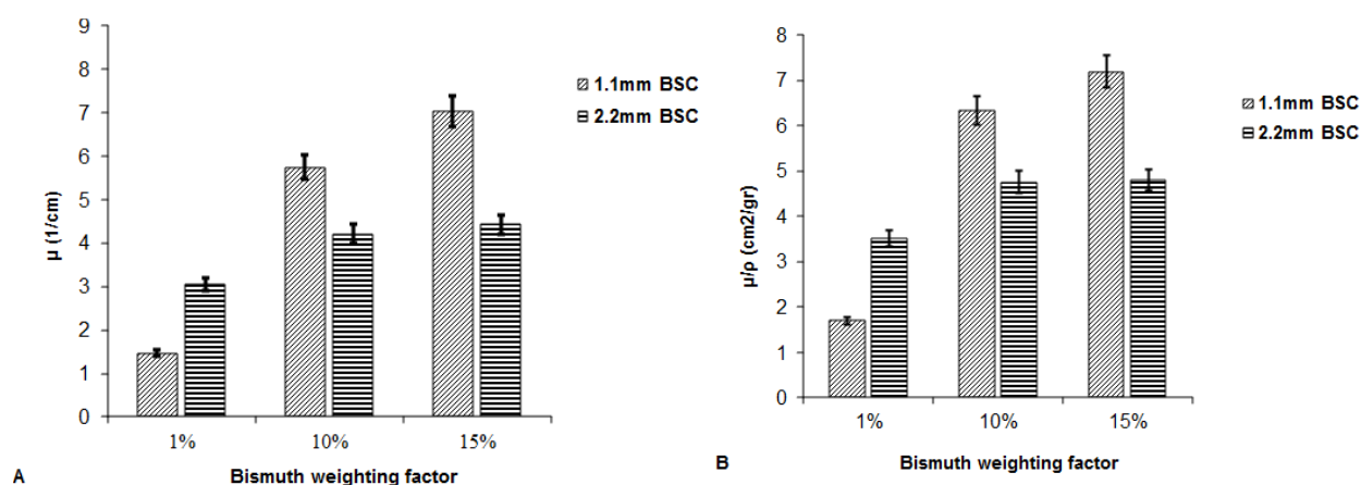
Figure 1. linear attenuation coefficient (μ, 1/cm). with (±SD) as shown in A. Mass attenuation coefficient (μ/ρ, cm 2 /gr), as shown in B for in BSC (Bismuth Silicone Composite) shields in 1.1 and 2.2 mm thicknesses on the chest phantom during Chest CT.
