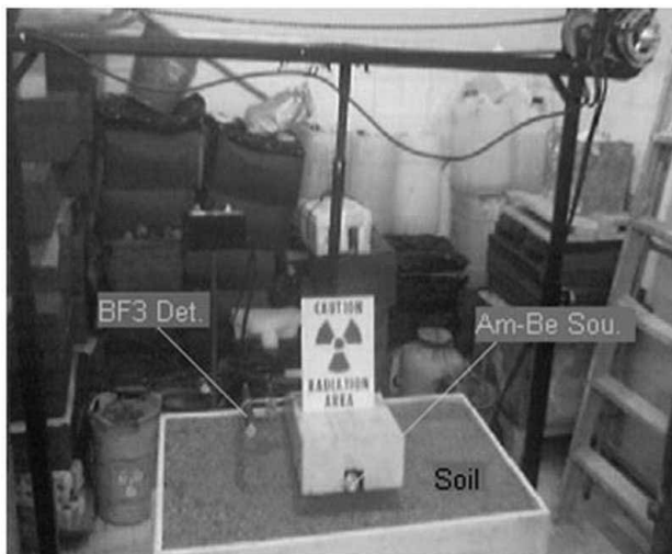
Figure 5. Photograph of landmine detection set-up.
