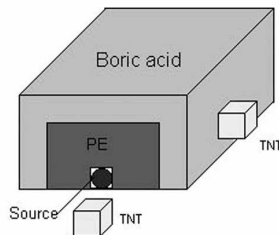
Figure 1. Locations of TNT samples, source and its shield with respect to each other in Monte Carlo simulation.
