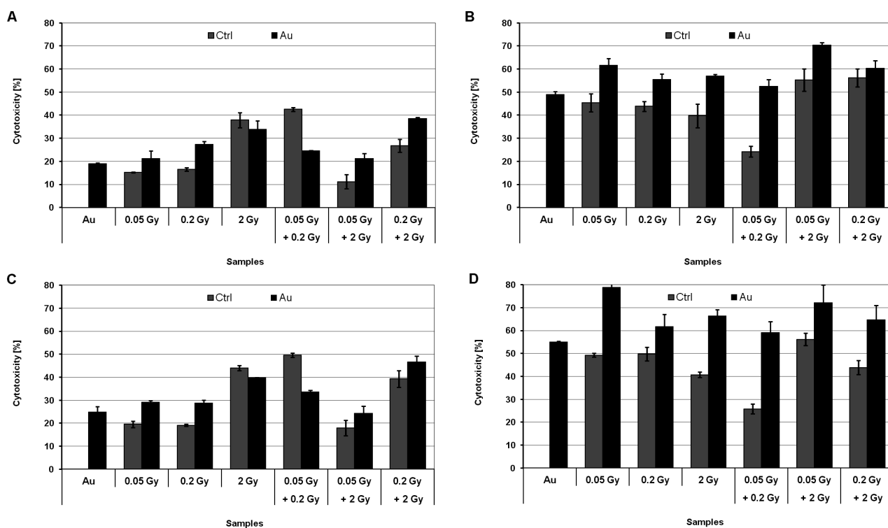
Figure 3. The cytotoxicity [%] measured in control (Ctrl) and samples treated with nAu/β-CD formulation (Au) of irradiated MRC-5 cells after 24 h recovery time (A), A549 cells after 24 h recovery time (B), MRC-5 cells after 72 h recovery time (C) and A549 cells after 72 h recovery time (D).
