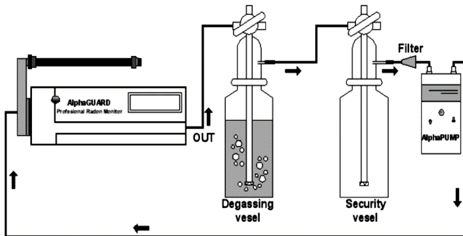
Figure 2. measurement system.
