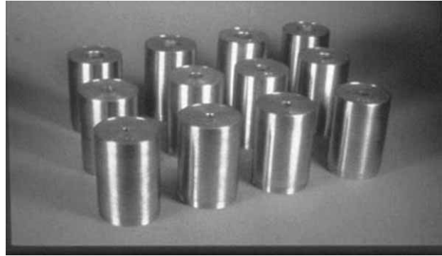
Figure 1. A set of 19 circular collimators from 5 mm to 50 mm in diameter at isocentre distance with 2.5 mm steps.
