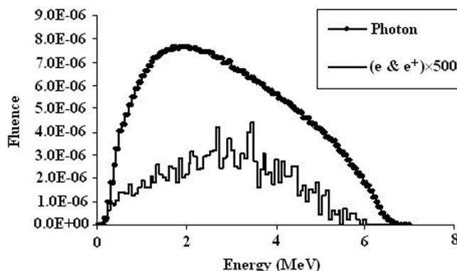
Figure 3. The photon, electron and positron energy spectra /MeV/ incident particle for a circular cone with 5 cm in diameter. Electrons and positrons spectra are multiplied by 500 to be shown on the same graph as for the photon spectra.
