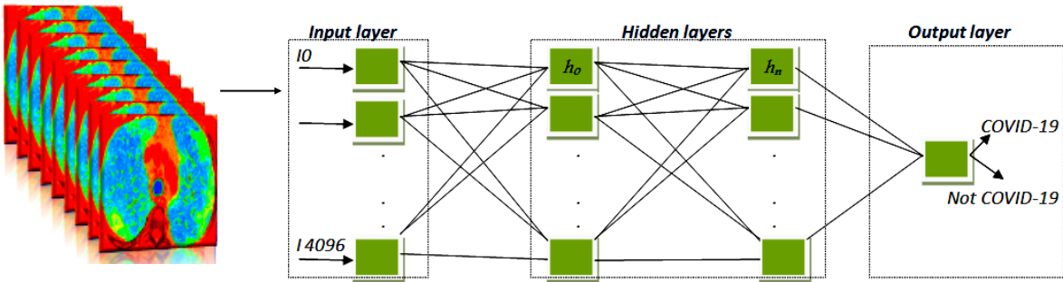
Figure 3. COVID-ANN architecture.
