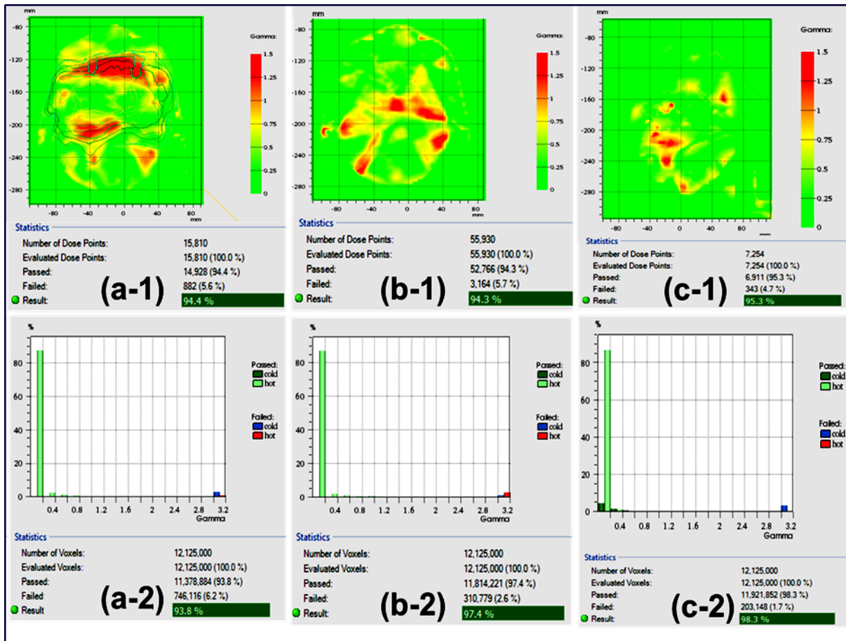
Figure 4. Comparison of 2D (a-1, b-1, c-1) and 3D (a-2, b-2, c-2) dose distribution between a) TPS and MC simulation with SOURCE 8, b) TPS and simulation with SOURCE 20, and c) simulation with SOURCE 8 and SOURCE 20 in the DOSXYZnrc.
