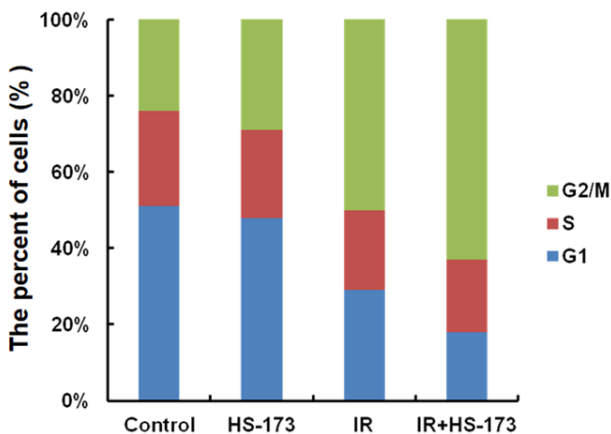
Figure 4. HS-173 triggered IR-induced cell cycle arrest at G2/M phase. MDA-MB-231 cells were treated with HS-173 (1 μM), irradiated with 5 Gy for 24 h, stained with PI, and analyzed through flow cytometry. Quantitative PI staining data is presented as a percentage of cell cycle distribution.
