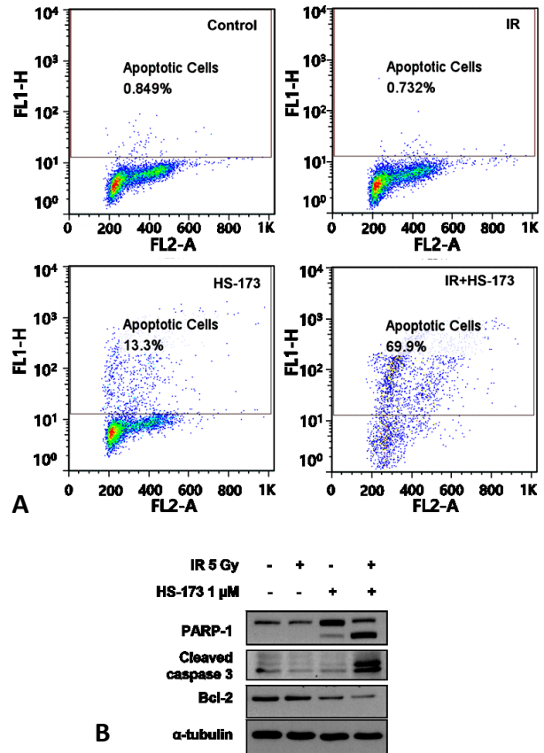
Figure 5. HS-173 sensitized MDA-MB-231 cells to irradiation. A. MDA-MB-231 cells were treated with HS-173 (1 μM) and irradiated with 5 Gy for 24 h. DNA fragmentation in MDA-MB-231 cells was evaluated through flow cytometry and TUNEL staining. B. Western blot analysis for apoptosis-related protein (PARP, cleaved caspase-3, and Bcl-2).
