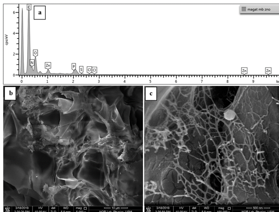
Figure 4. FESEM-EDX micrographs of MAGAT added with methylene blue and ZnO (a) EDX data, and the FESEM micrographs at (b) 5000× and (c) 100000×.
