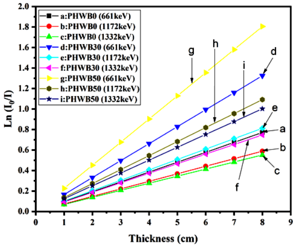
Figure 3. Ln (I 0 /I) against thicknesses for the phthalonitrile/WB samples at Cs-137 and Co-60 energy sources.
