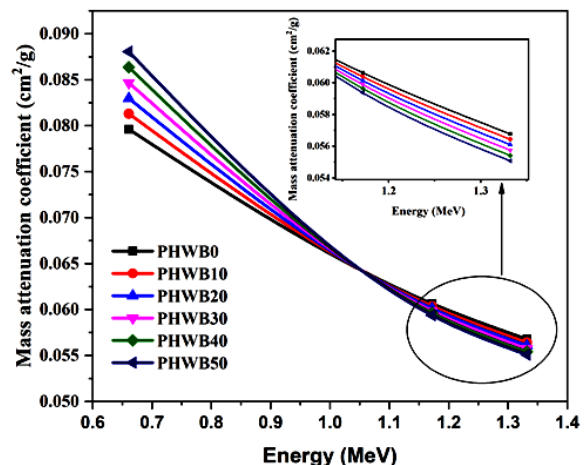
Figure 2. Mass attenuation coefficients using XCOM for PHWB samples versus energy sources.
