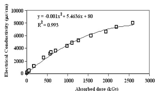
Figure 2. Dose response of SED at high dose range 0 - 2592 kGy using 60 Co gamma radiation at 5.969 kGy/h.
