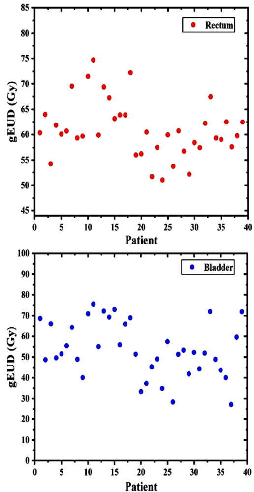
Figure 4. Estimated gEUD values inside the bladder and rectum for all studied patients.
