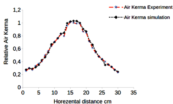
Figure 3. The results of body bowtie filter thicknesses.
