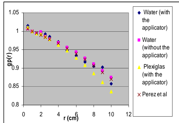
Figure 3. Comparison of the radial dose function of a single pellet source with and without the applicator in water and plexiglas phantoms.
