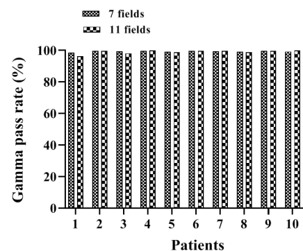
Figure 2. The percentage of gamma passing rate (obtained by the TPS and phantom) for both 7 and 11 fields.
