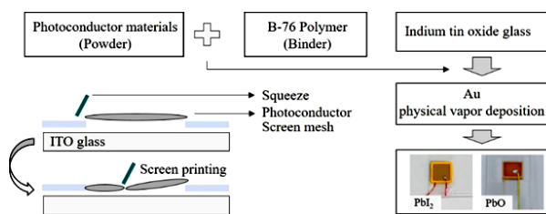
Figure 1. Fabrication process of polycrystalline semiconductor dosimeter using PbI 2 and PbO materials.
