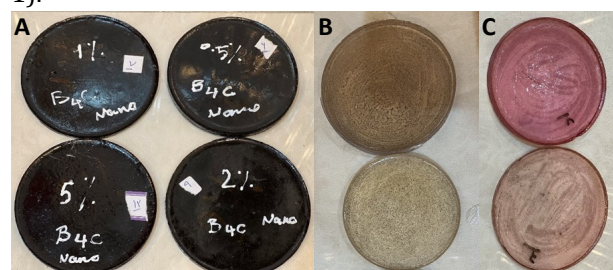
Figure 1. The prepared polyester/boron carbide(B 4 C) composites with (a) nano-B 4 C and (b) micro-B 4 C. (c) The control samples (pure polyesters) are shown on the right side.
